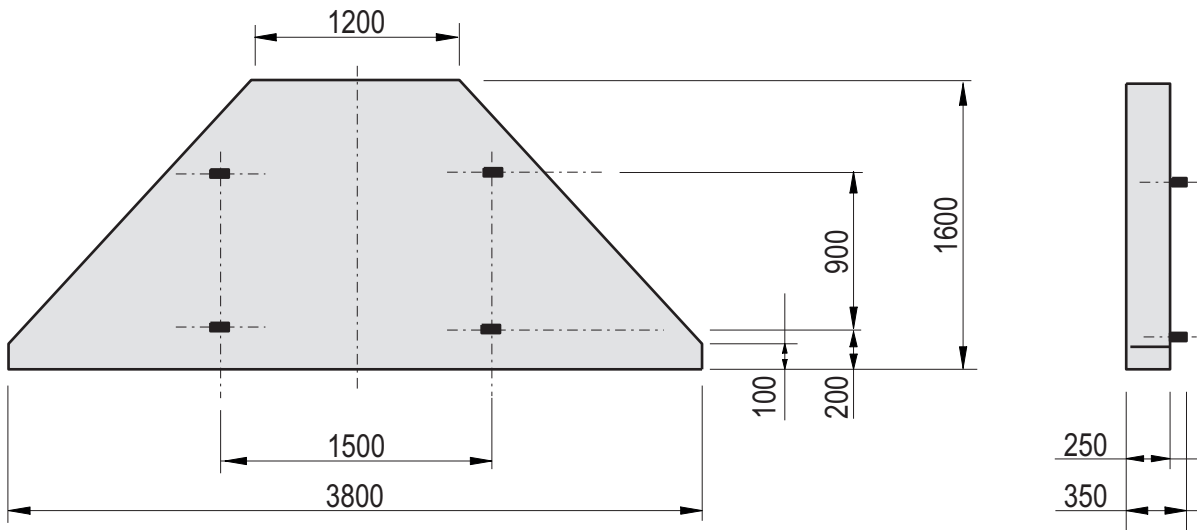
Central ballast block ZB 2.5, Art.-Nr.: 30021891
