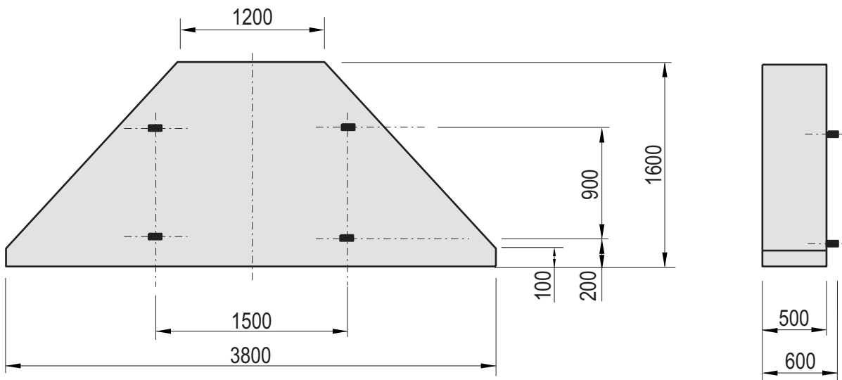
Central ballast block ZB 5, Art.-Nr.: 30021890
